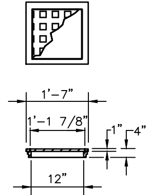
SUMP FRAME & GRATE
