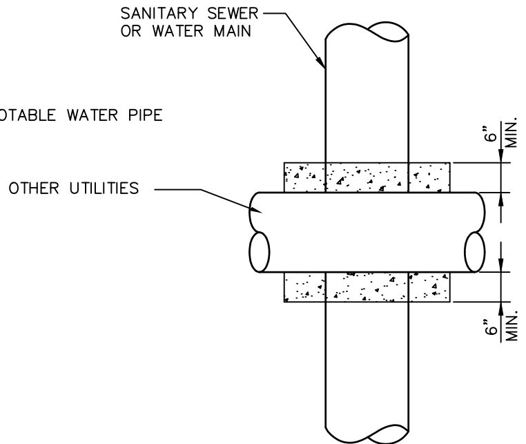
UTILITY CROSSINGS
