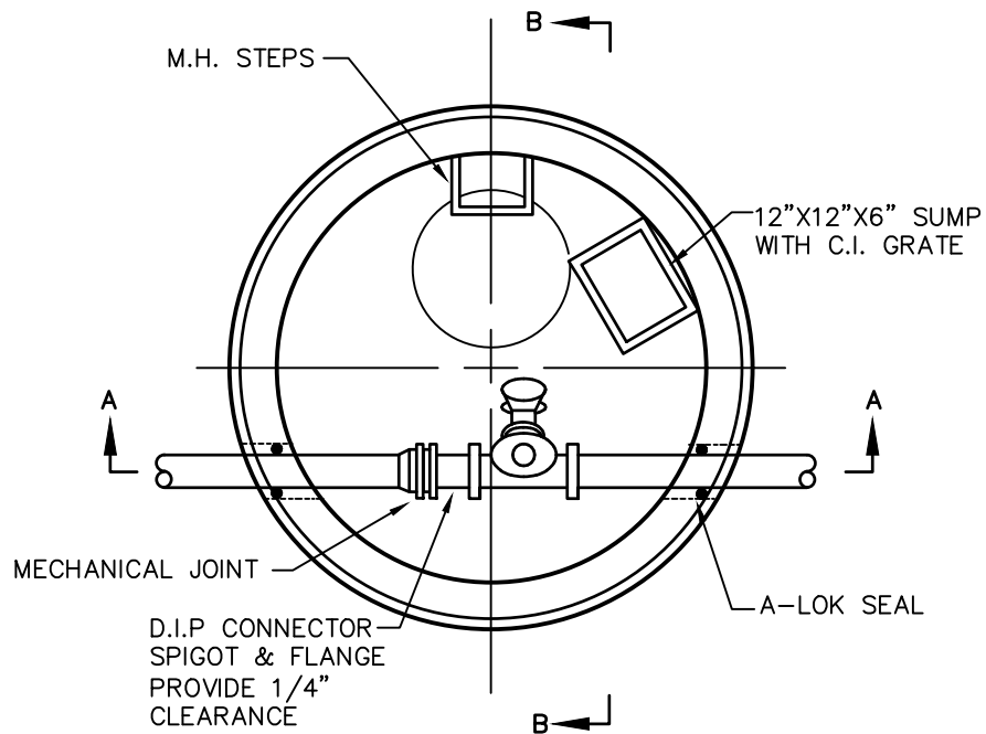
PLAN SECTION
