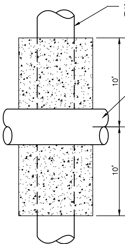
WATER CROSSINGS
