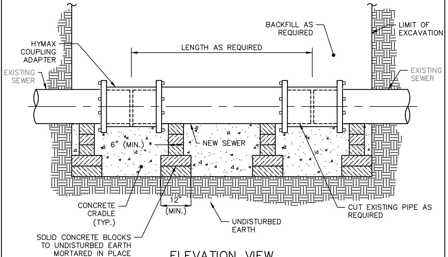
ELEVATION VIEW
